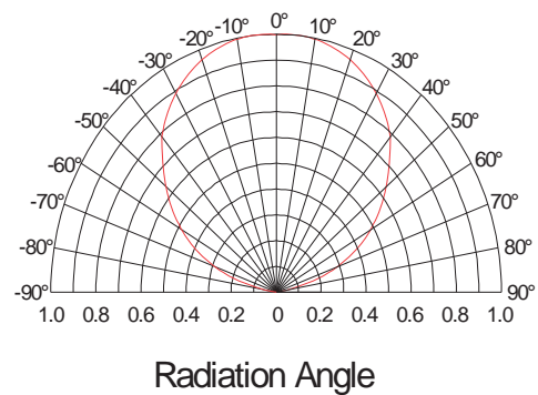
Radiation Characteristics
